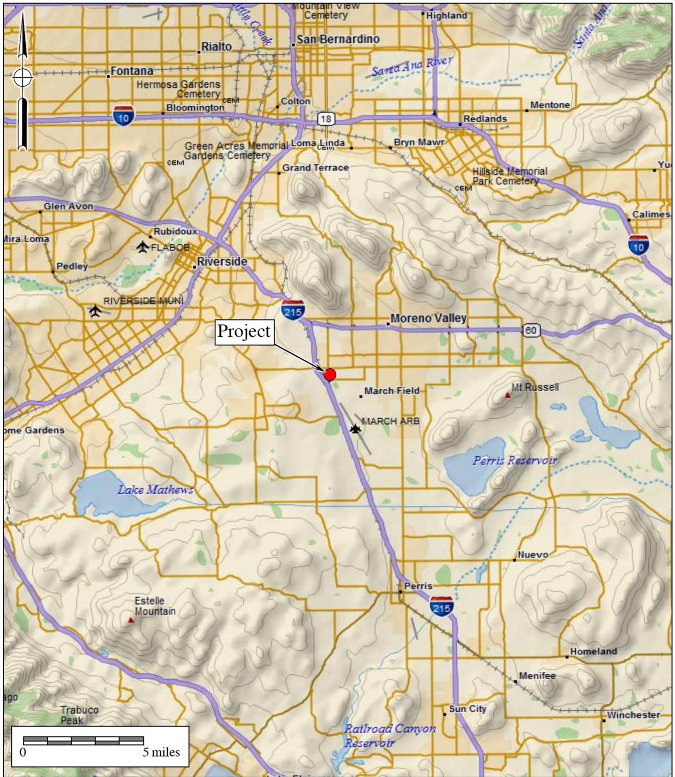
Figure 1 General Location Map The First Day Street Logistics Project DeLorme (1:250,000)
