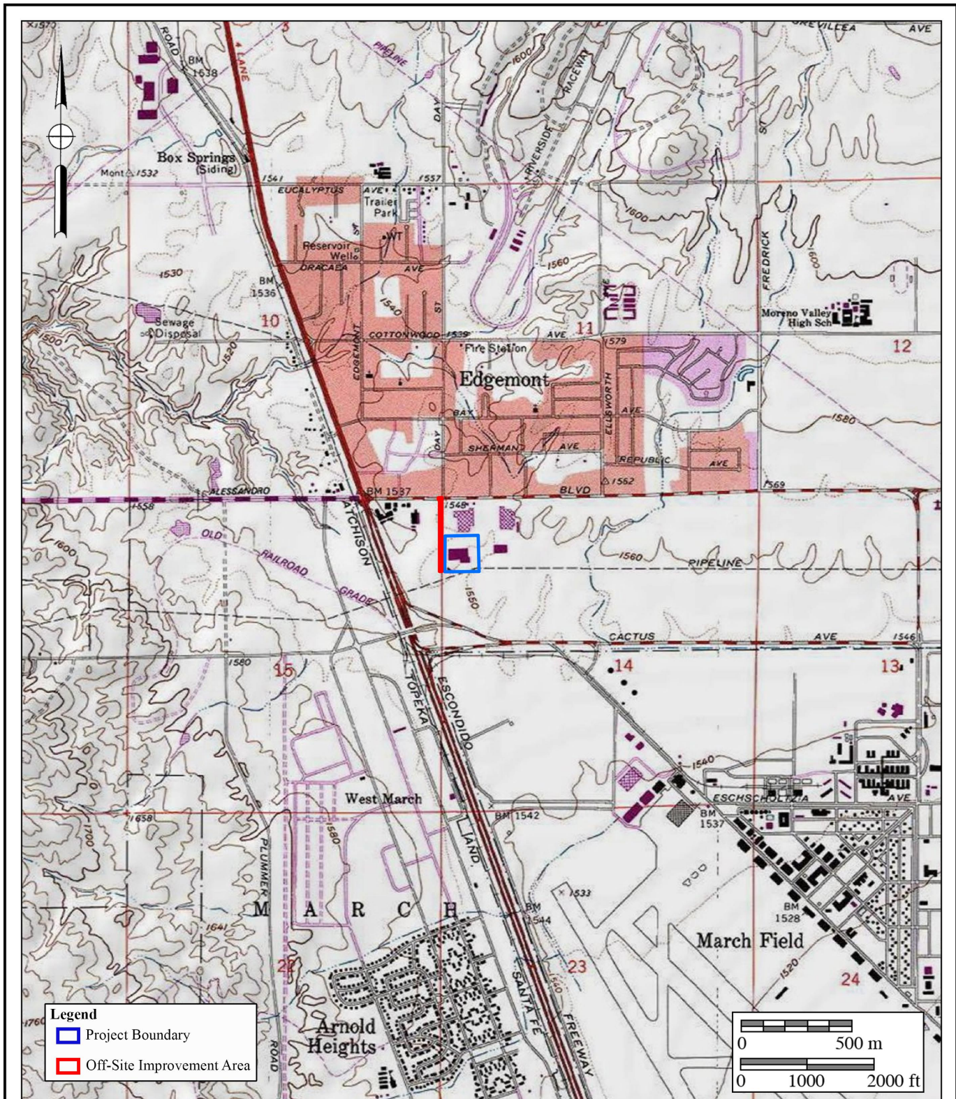
Figure 2 Project Location Map The First Day Street Logistics Project USGS Riverside East Quadrangle (7.5-minute series)
