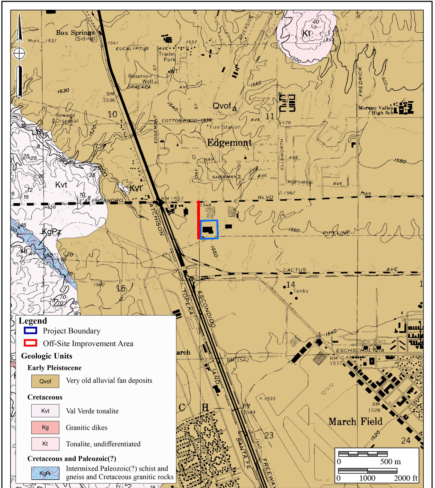
Figure 3 Geologic Map
